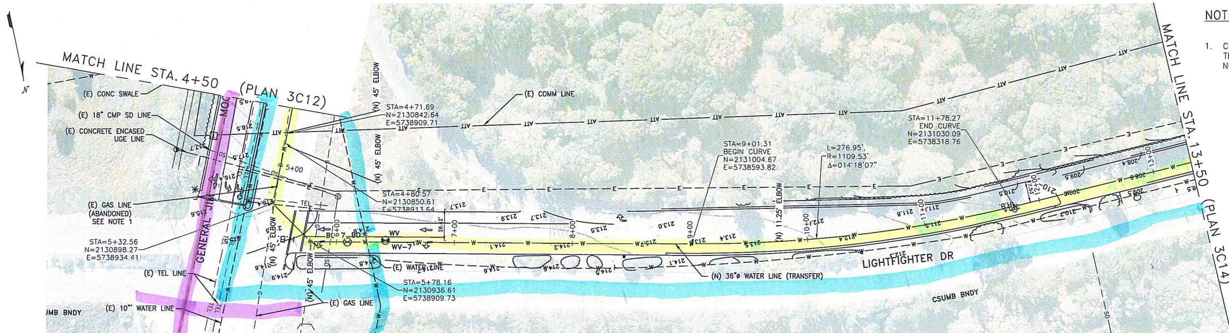
PLAN 1"=40'
