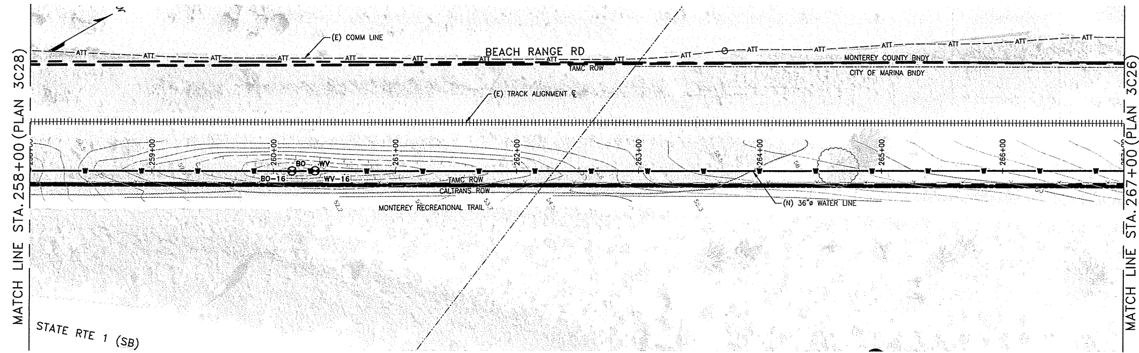
PLAN 1"=40'
