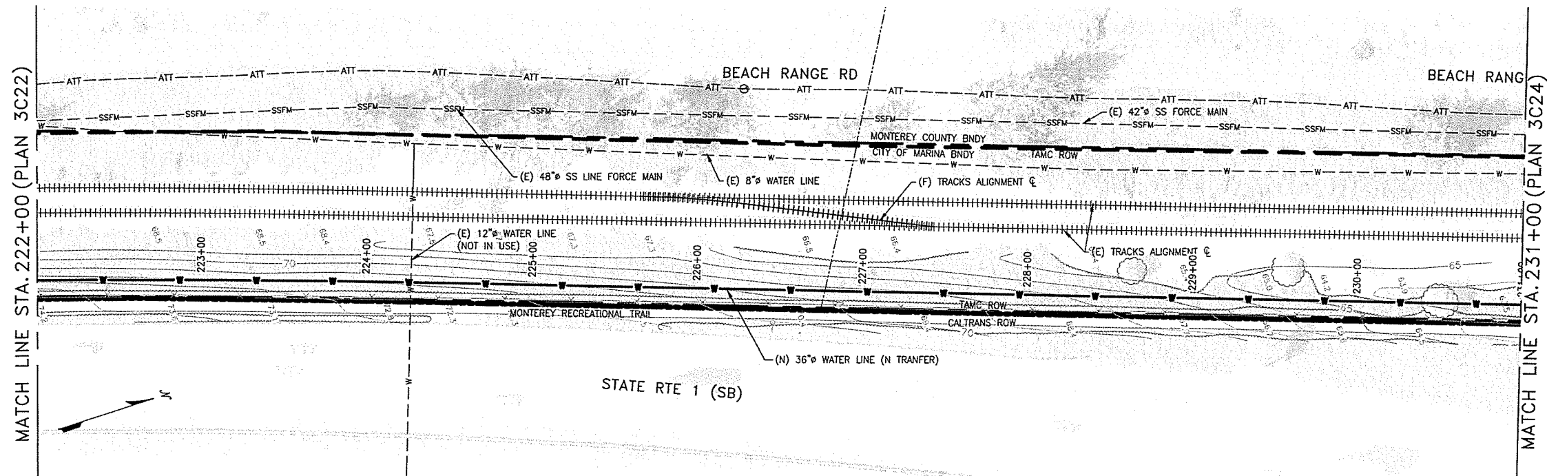
PLAN 1"=40'
